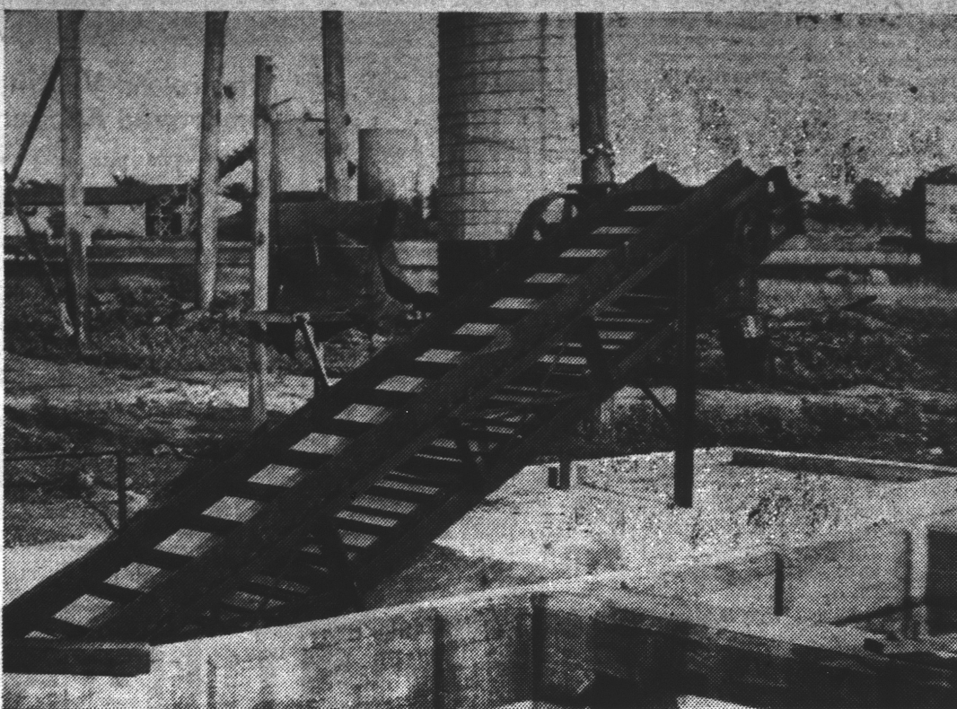
Screening is the first step in the operations at the model plant for treatment and disposal of waste. Above is shown the screen which eliminates bulkier waste material from liquids. The model plant was developed in an attempt to solve the problem of stream pollution.
