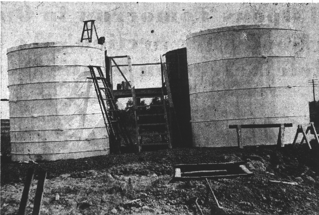
Two of the tanks used at the model Greenwood plant of Stokley Brothers & Co. in an effort to end stream pollution from cannery wastes are shown above. Two sets of settling tanks play an important part in the operation of the system, engineers declare.
