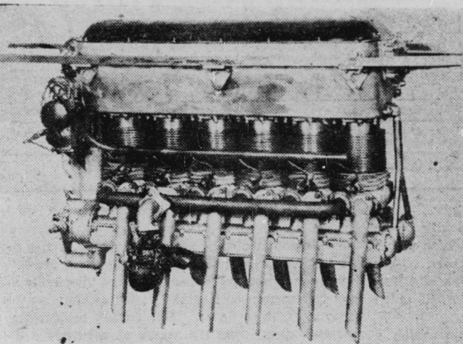
Photo shows the new six-cylinder airplane motor manufactured by the Arthur Chevrolet Aviation Motors Corporation of Indianapolis which has been approved by the department of commerce. The motor is known as the "Chevolair."
