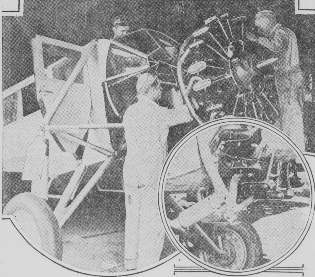
Lindbergh's new monoplane is shown here receiving its air-cooled power plant, known in flying parlance as a Wright Radial J-5-C. Note the windows in the front of the fuselage; these will give the pilot much wider visibility than his old ship. Inset offers a detailed view of the landing gear, brakes on the wheels and the manifold heater which will warm the closed cabin.
