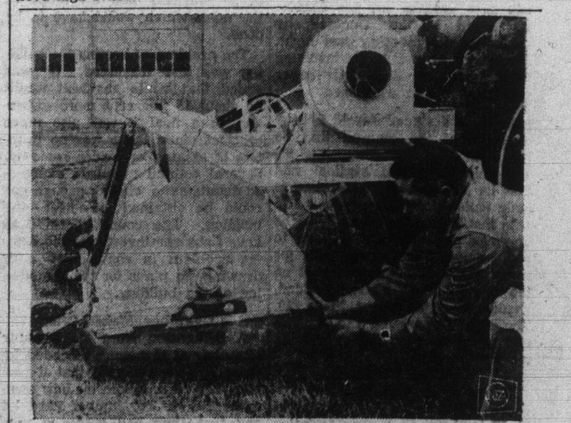
BEATS THE WEEVIL PROBLEM—Ready for field testing this summer, experimental vacuum-beater, above, picks up larvae-infested cotton flower buds that have fallen to the ground, pulverizes them with a flailing mechanism, and blows the debris back on the ground. Its use would eliminate the hand-gathering used at present to clear infested fields. Machine's designer, Eddie C. Burt, Agricultural Research Service engineer, readies the machine for tests at Boll Weevil Research Laboratory, State College, Miss.
