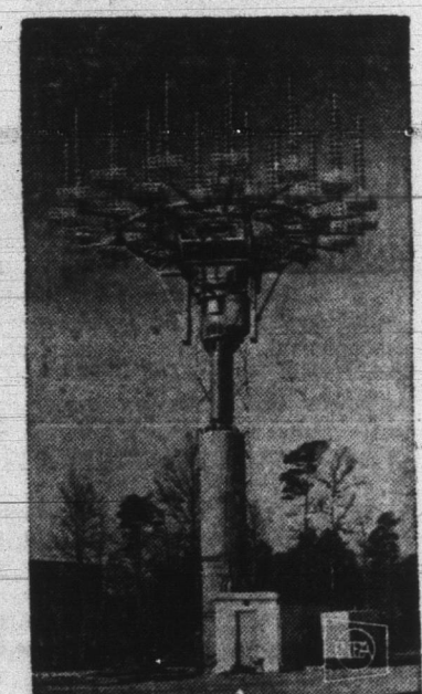
ROCKET RADIO —Looking like an electronics-age candleabra, this is a high-gain telemetry antenna at Wallops Island, Va. It's used for receiving signals from high-altitude payloads on rockets.
