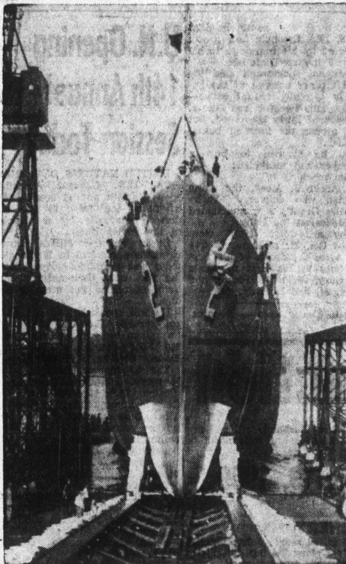
FIRST BUILT FROM KEEL UP —The guided missile destroyer Charles F. Adams, named for the late Navy secretary, is launched at Bath Iron Works, Bath, Me. It is the first built from the keel up as a guided missile destroyer. Armament includes the Tartar Twin missile system, highly effective against low or high targets.
